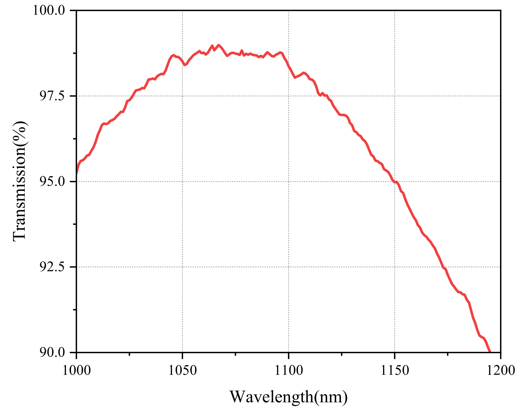
Transmission of VBE-1064-2-10X
