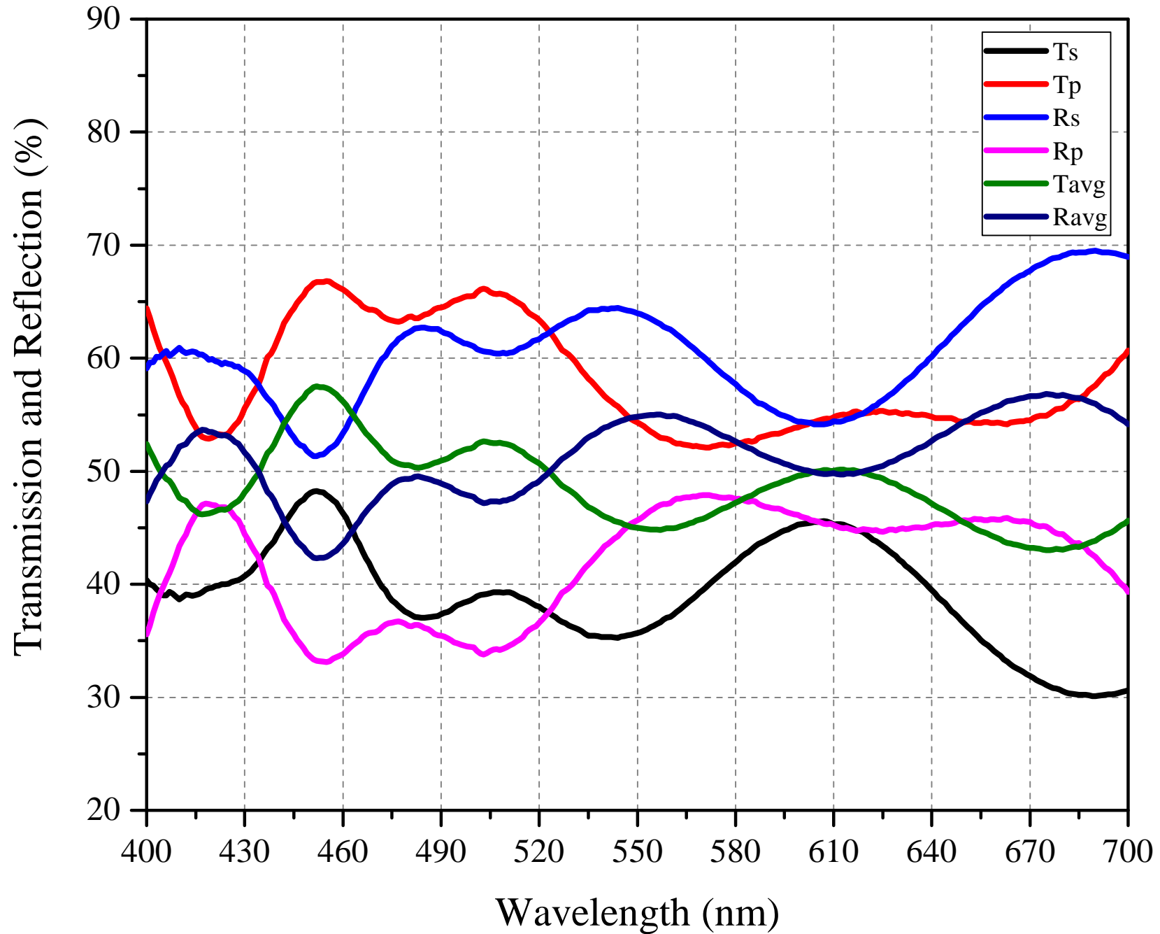
50:50 Plate Beamsplitter Transmission and Reflection (AR Coating: 400 nm-700 nm)
