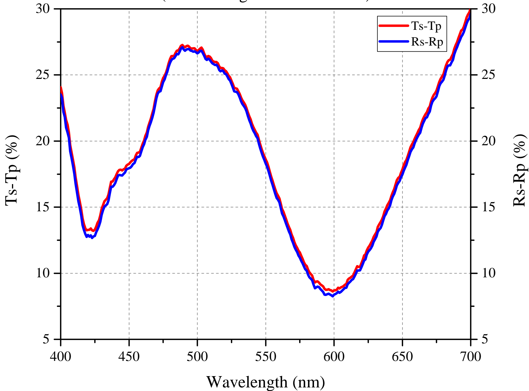
50:50 Plate Beamsplitter Ts-Tp and Rs-Rp (AR Coating: 400 nm-700 nm)
